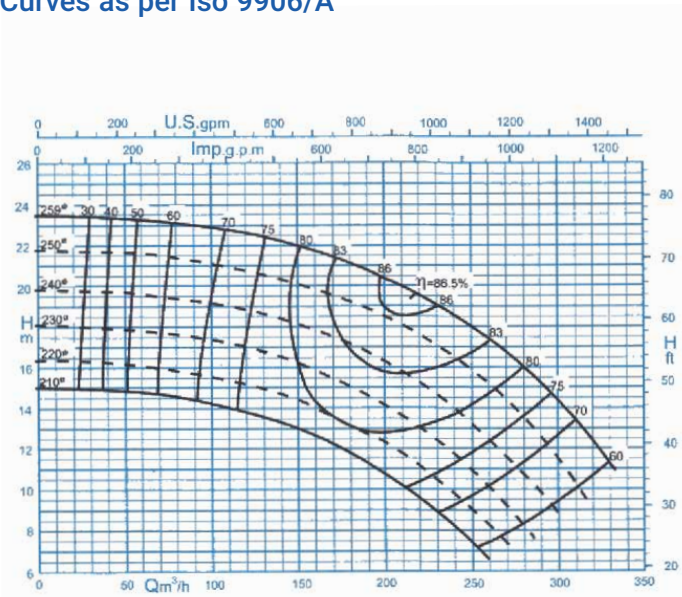
Curves as per Iso 9906/A
